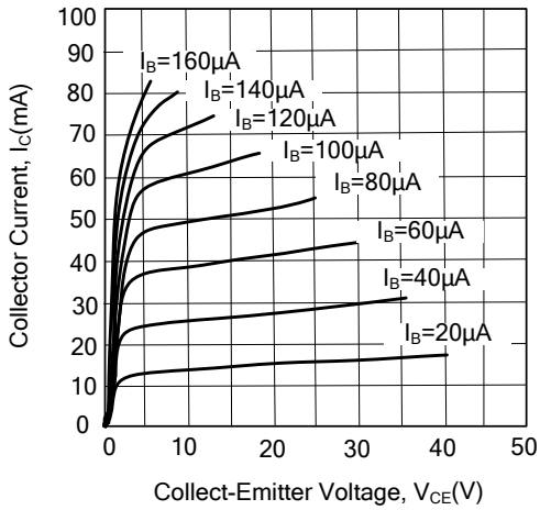
Static Characteristic
