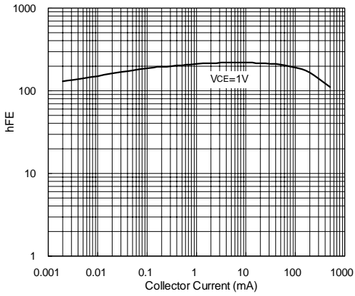
FIG.1 - Current Gain & Collector Current
